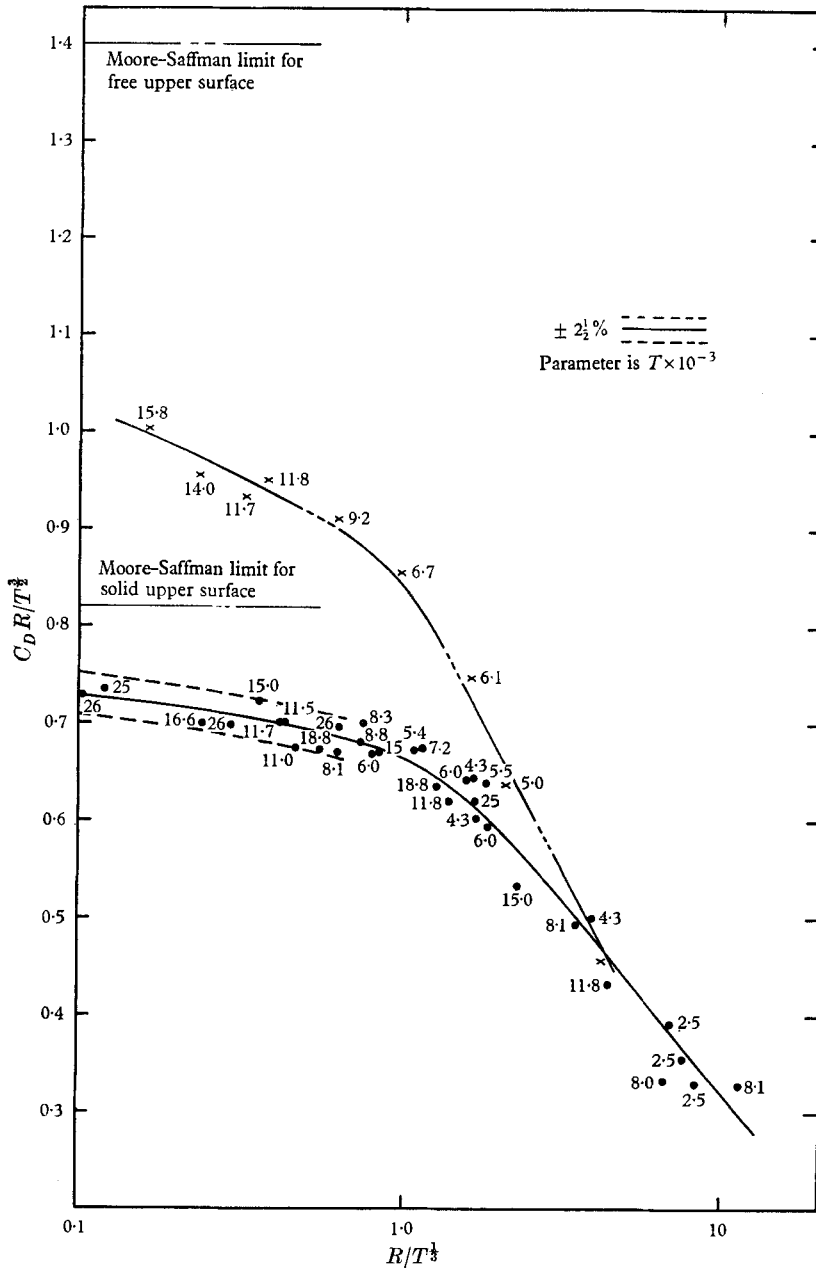
FIGURE 3. C_D R/T^{3/2} versus R/T^{3/2} ; the best data reduction found to show the approach to results dominated by viscous and Coriolis forces.
