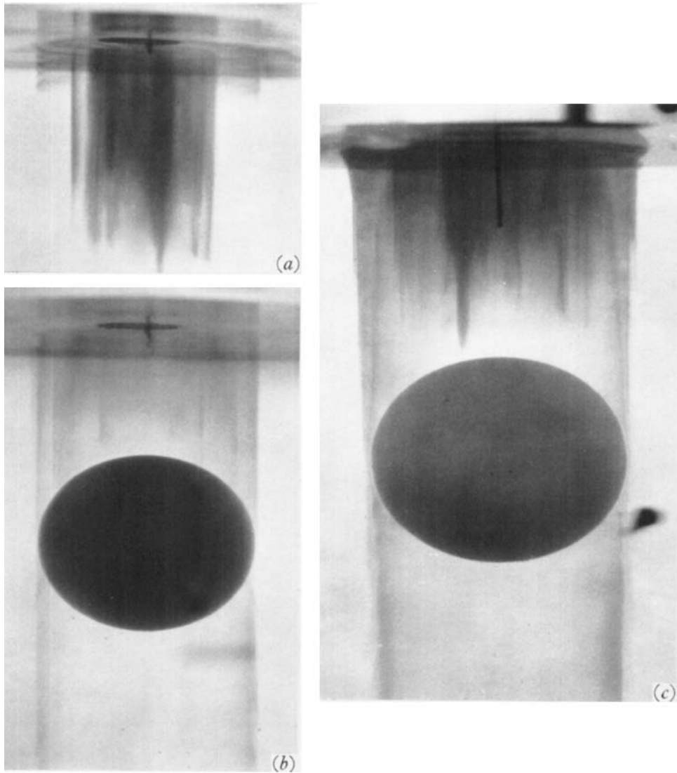
FIGURE 6(a) and (b). The change in the shape of a dye column introduced ahead of a rising sphere. Note the dye flow away from the upper wall in (a), and the change in diameter of the column of dye. T = 12,000 ; R = 9.5 . (c). Showing a thinning of the shear layer and the clear division between fluid in this layer and that within the central region. T = 8400 ; R = 15.5 .
