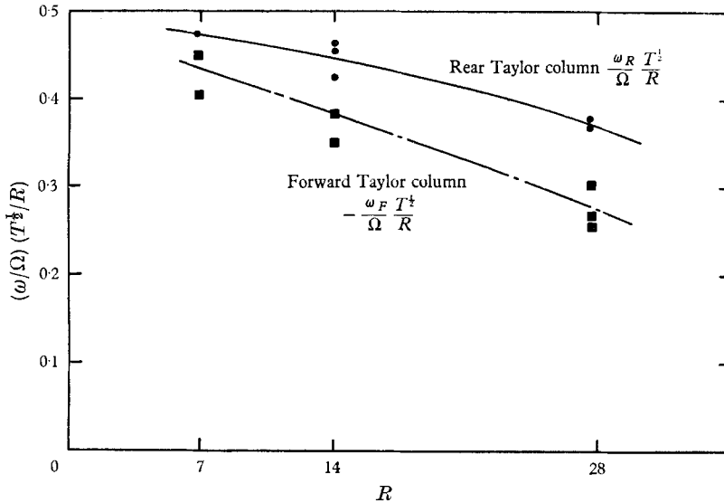
FIGURE 10. (\omega/\Omega)(T^{1/2}/R) versus R for 4000 < T < 16,000 . The rotation rate of both fore ( -w_f ) and aft ( w_R ) slugs compared to the theoretically predicted value. \Omega is direction of positive rotation.
